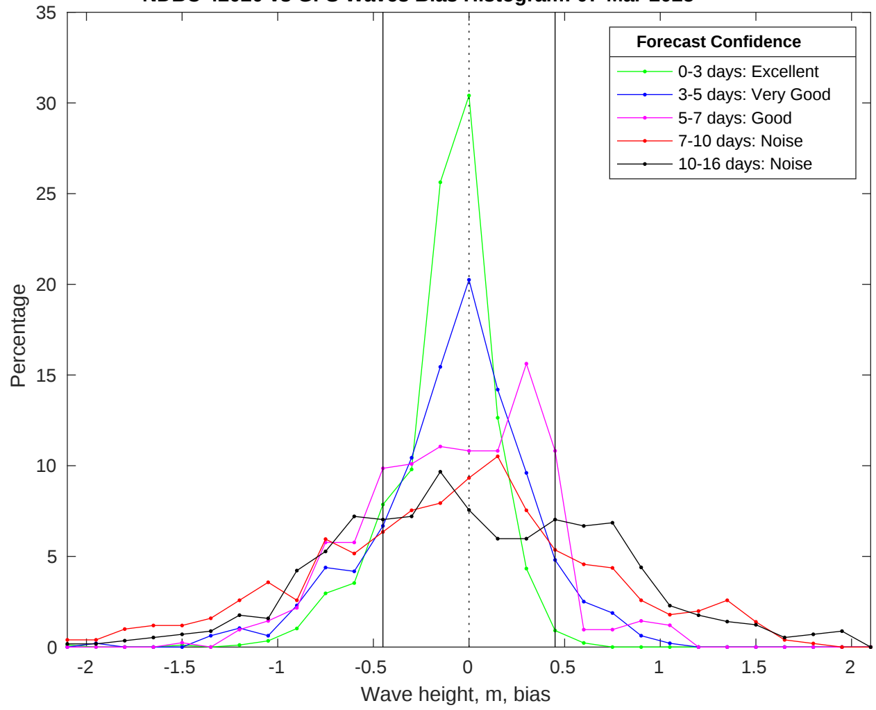
NDBC 42020 vs GFS Waves Bias Histogram: 07-Mar-2025
