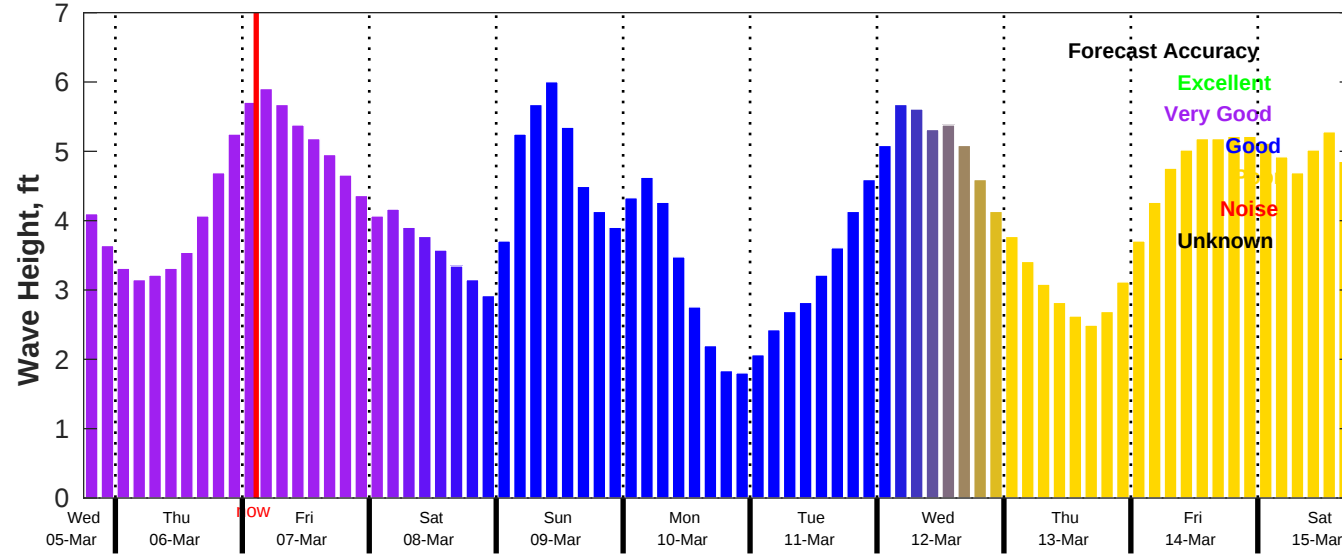
CMEMS Wave Forecast for NDBC 42020 from 05-Mar-2025 18:00:00 to 15-Mar-2025 18:00:00
