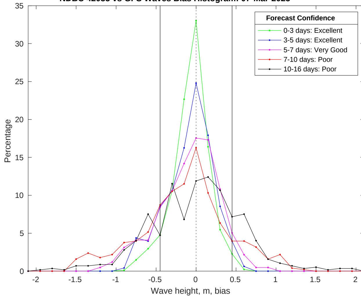
NDBC 42035 vs GFS Waves Bias Histogram: 07-Mar-2025
