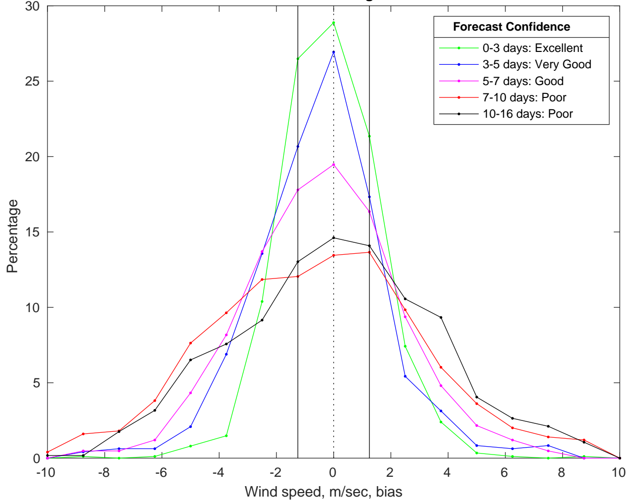
NDBC 42035 vs GFS Winds Bias Histogram: 07-Mar-2025
