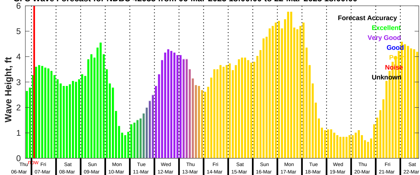
GFS Wave Forecast for NDBC 42035 from 06-Mar-2025 18:00:00 to 22-Mar-2025 18:00:00
