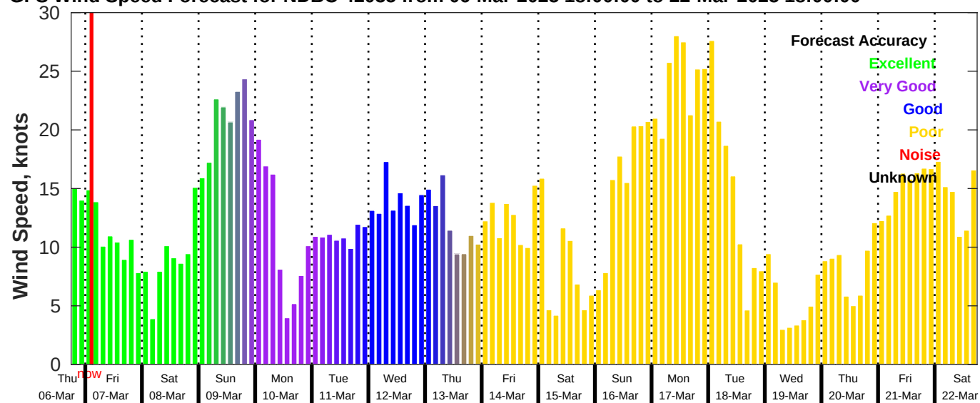
GFS Wind Speed Forecast for NDBC 42035 from 06-Mar-2025 18:00:00 to 22-Mar-2025 18:00:00
