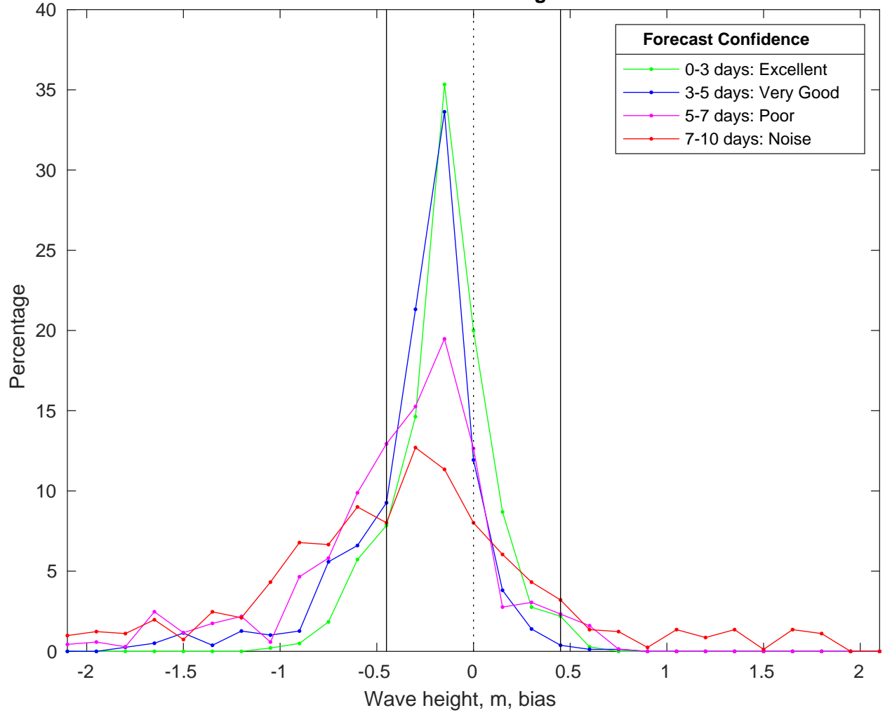
NDBC 42036 vs CMEMS Waves Bias Histogram: 07-Mar-2025
