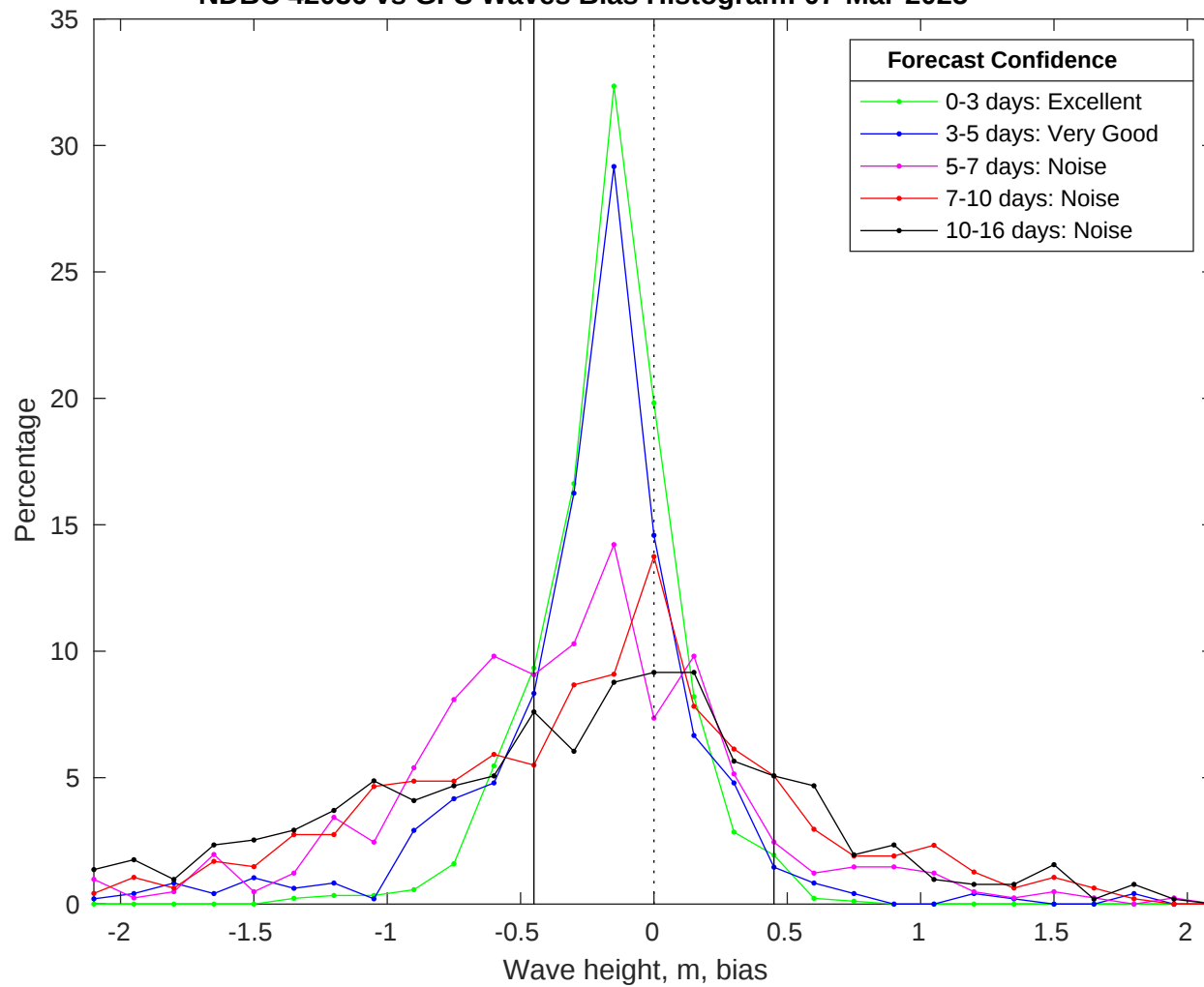
NDBC 42036 vs GFS Waves Bias Histogram: 07-Mar-2025
