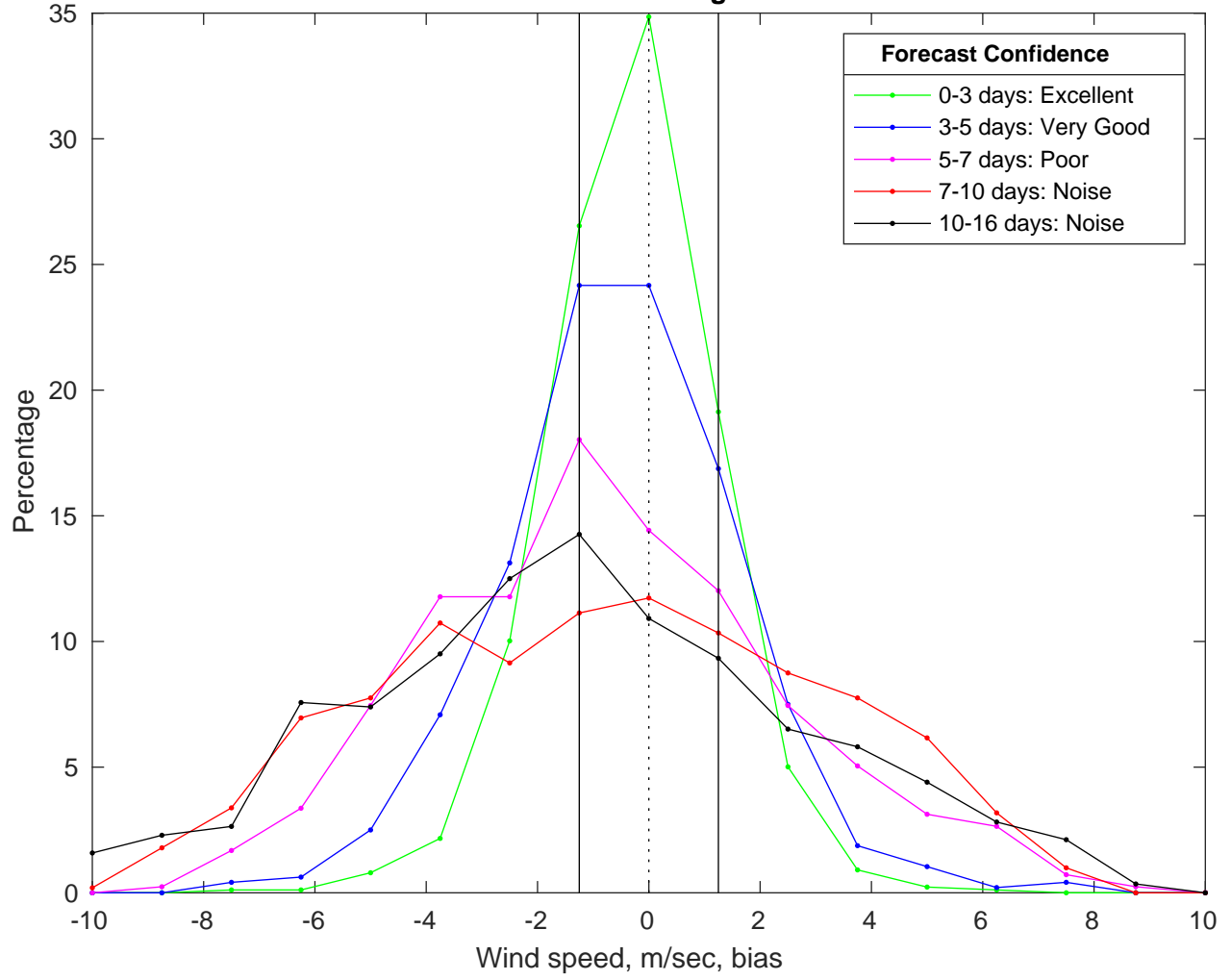
NDBC 42036 vs GFS Winds Bias Histogram: 07-Mar-2025
