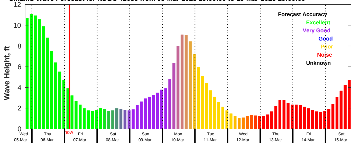
CMEMS Wave Forecast for NDBC 42036 from 05-Mar-2025 19:00:00 to 15-Mar-2025 19:00:00
