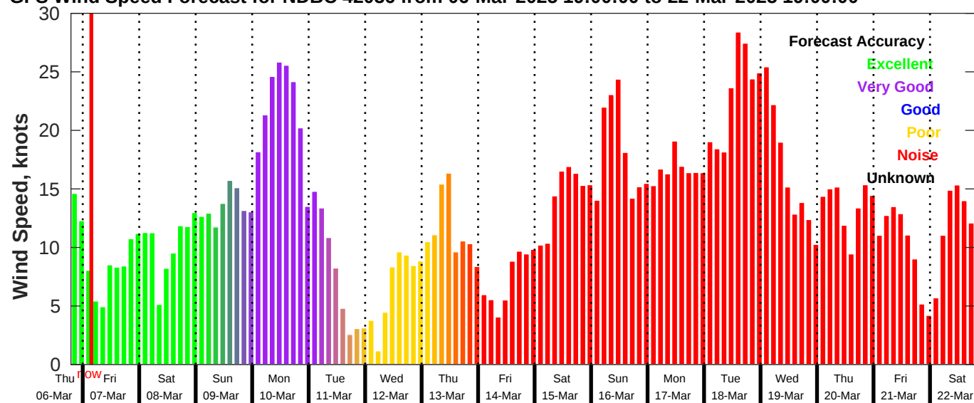
GFS Wind Speed Forecast for NDBC 42036 from 06-Mar-2025 19:00:00 to 22-Mar-2025 19:00:00
