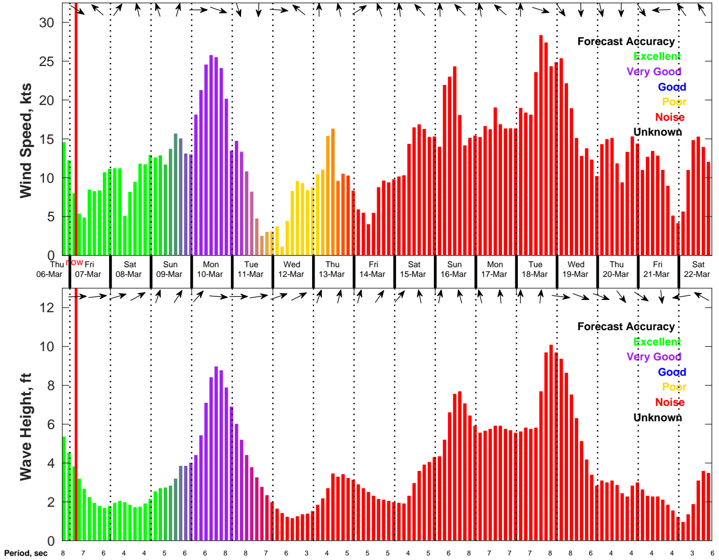
Wind & Wave Forecast for NDBC 42036 from 06-Mar-2025 19:00:00 to 22-Mar-2025 19:00:00
