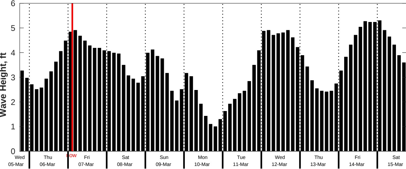
CMEMS Wave Forecast for NDBC 42092 from 05-Mar-2025 18:00:00 to 15-Mar-2025 18:00:00
