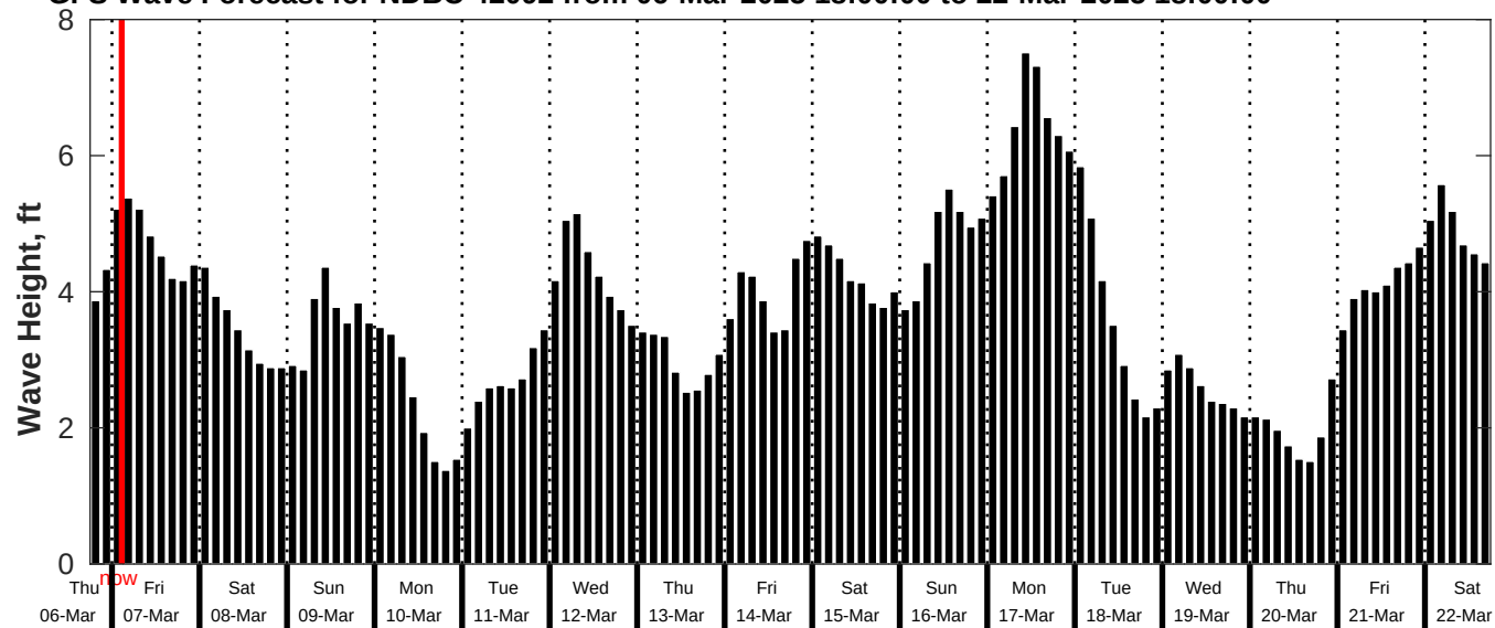
GFS Wave Forecast for NDBC 42092 from 06-Mar-2025 18:00:00 to 22-Mar-2025 18:00:00
