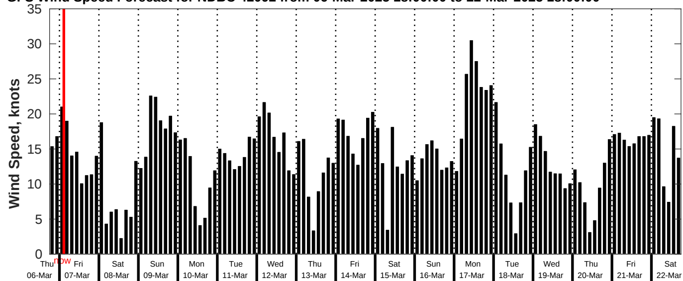
GFS Wind Speed Forecast for NDBC 42092 from 06-Mar-2025 18:00:00 to 22-Mar-2025 18:00:00
