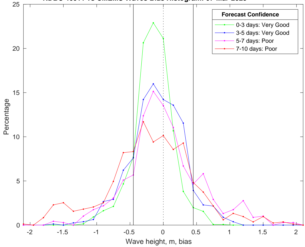
NDBC 46011 vs CMEMS Waves Bias Histogram: 07-Mar-2025
