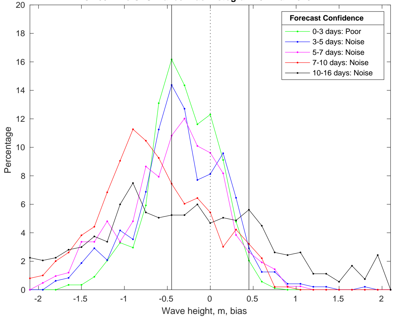
NDBC 46011 vs GFS Waves Bias Histogram: 07-Mar-2025
