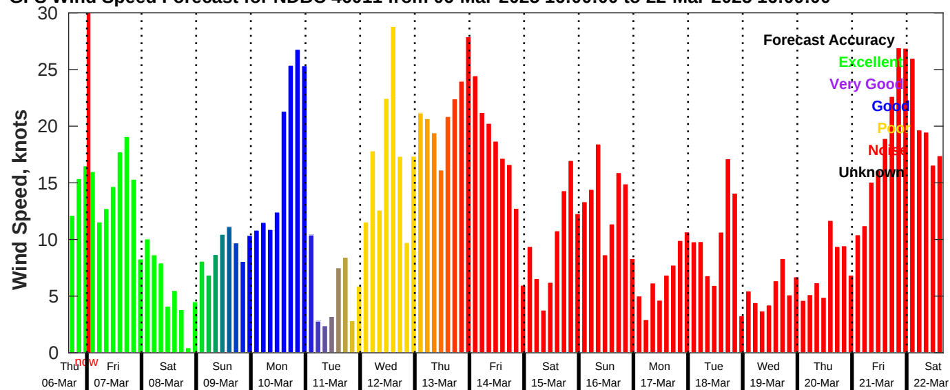
GFS Wind Speed Forecast for NDBC 46011 from 06-Mar-2025 16:00:00 to 22-Mar-2025 16:00:00
