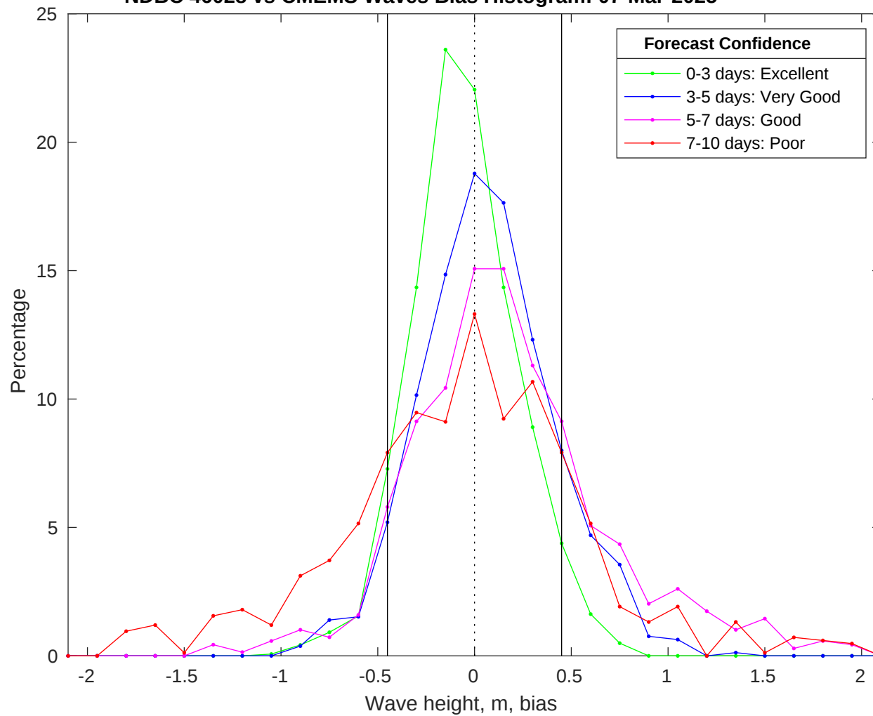
NDBC 46028 vs CMEMS Waves Bias Histogram: 07-Mar-2025
