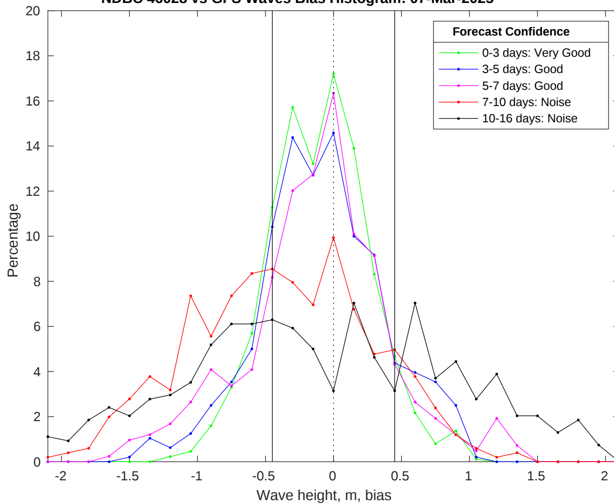
NDBC 46028 vs GFS Waves Bias Histogram: 07-Mar-2025
