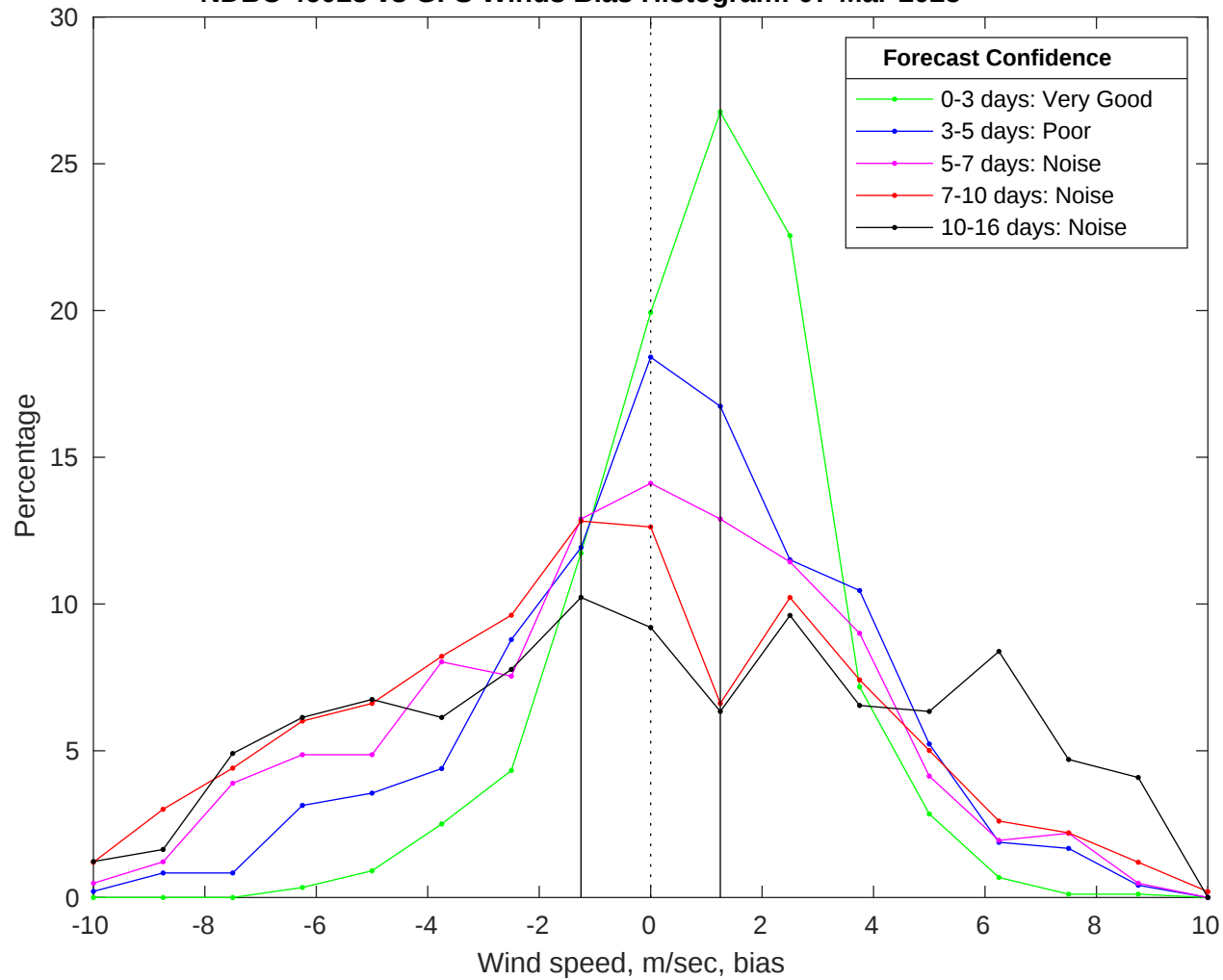
NDBC 46028 vs GFS Winds Bias Histogram: 07-Mar-2025
