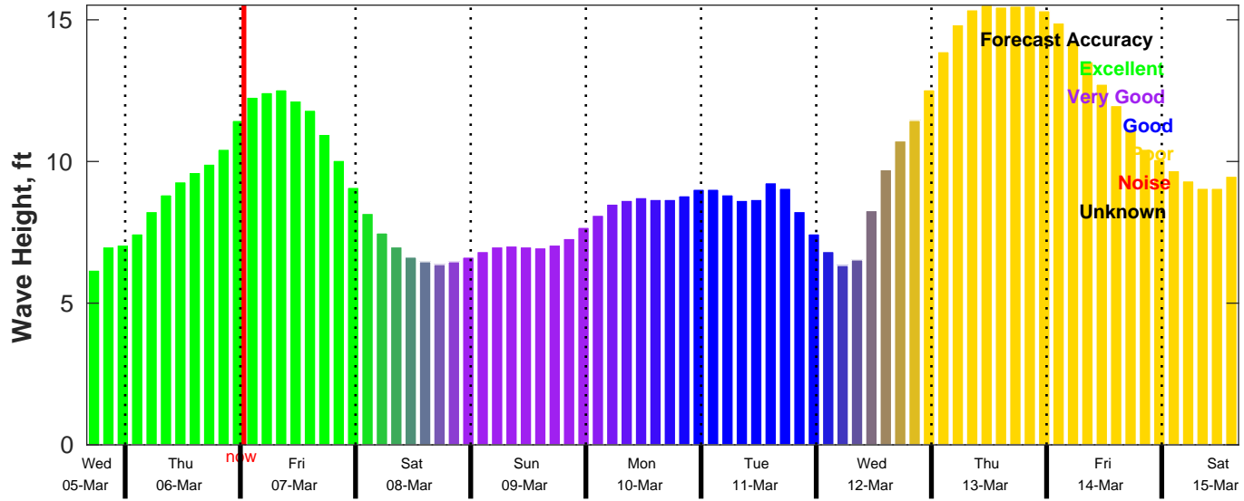
CMEMS Wave Forecast for NDBC 46028 from 05-Mar-2025 16:00:00 to 15-Mar-2025 16:00:00
