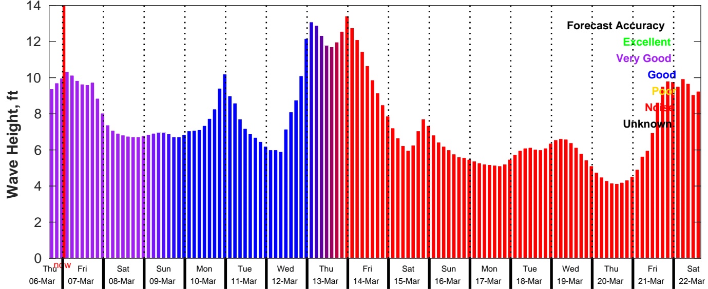
GFS Wave Forecast for NDBC 46028 from 06-Mar-2025 16:00:00 to 22-Mar-2025 16:00:00
