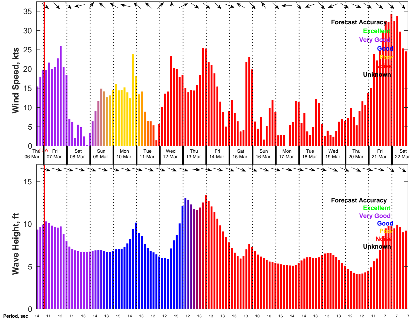
Wind & Wave Forecast for NDBC 46028 from 06-Mar-2025 16:00:00 to 22-Mar-2025 16:00:00
