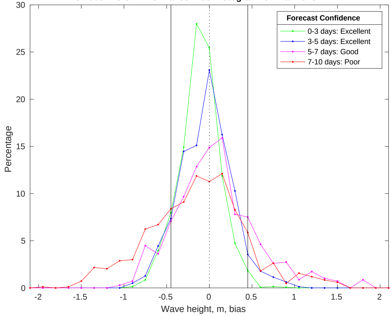
NDBC 46054 vs CMEMS Waves Bias Histogram: 07-Mar-2025
