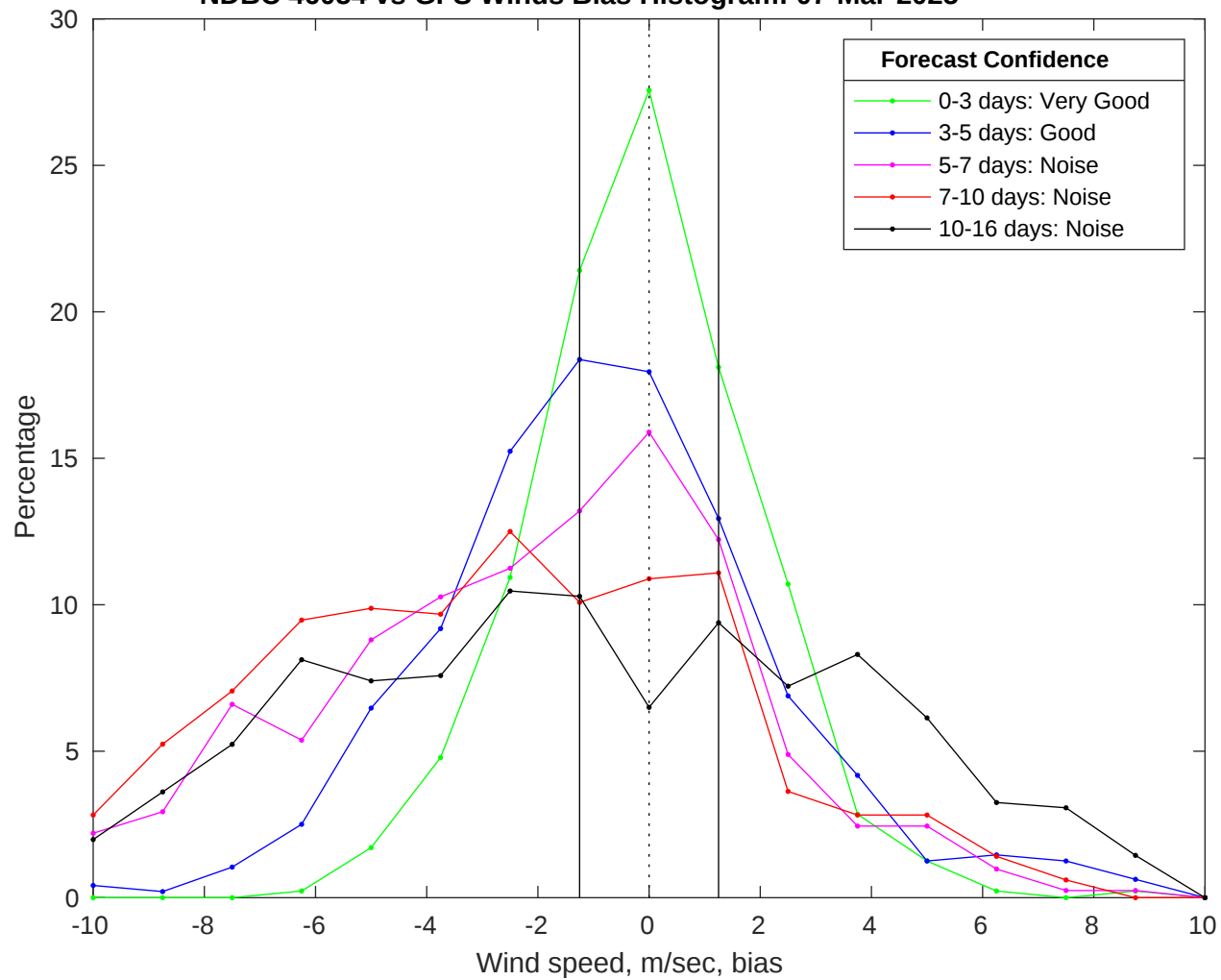
NDBC 46054 vs GFS Winds Bias Histogram: 07-Mar-2025
