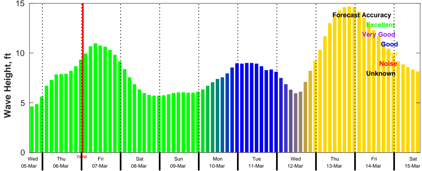
CMEMS Wave Forecast for NDBC 46054 from 05-Mar-2025 16:00:00 to 15-Mar-2025 16:00:00
