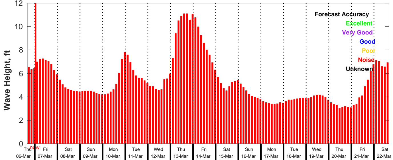
GFS Wave Forecast for NDBC 46054 from 06-Mar-2025 16:00:00 to 22-Mar-2025 16:00:00
