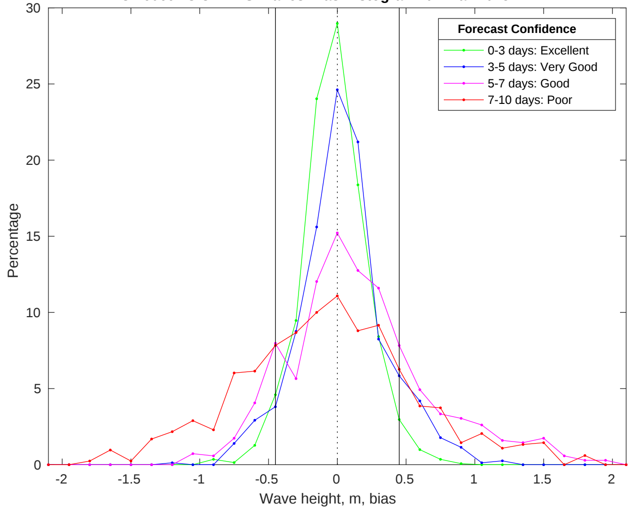
NDBC 46069 vs CMEMS Waves Bias Histogram: 07-Mar-2025
