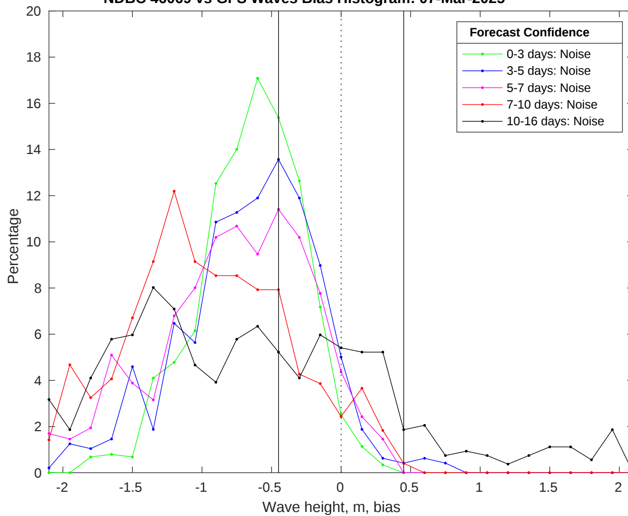
NDBC 46069 vs GFS Waves Bias Histogram: 07-Mar-2025
