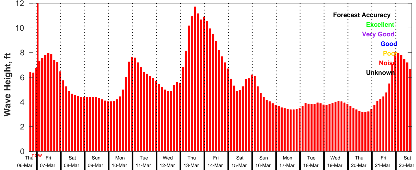
GFS Wave Forecast for NDBC 46069 from 06-Mar-2025 16:00:00 to 22-Mar-2025 16:00:00
