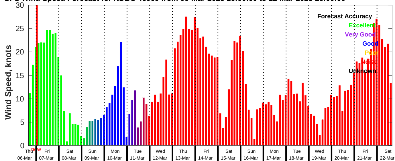
GFS Wind Speed Forecast for NDBC 46069 from 06-Mar-2025 16:00:00 to 22-Mar-2025 16:00:00
