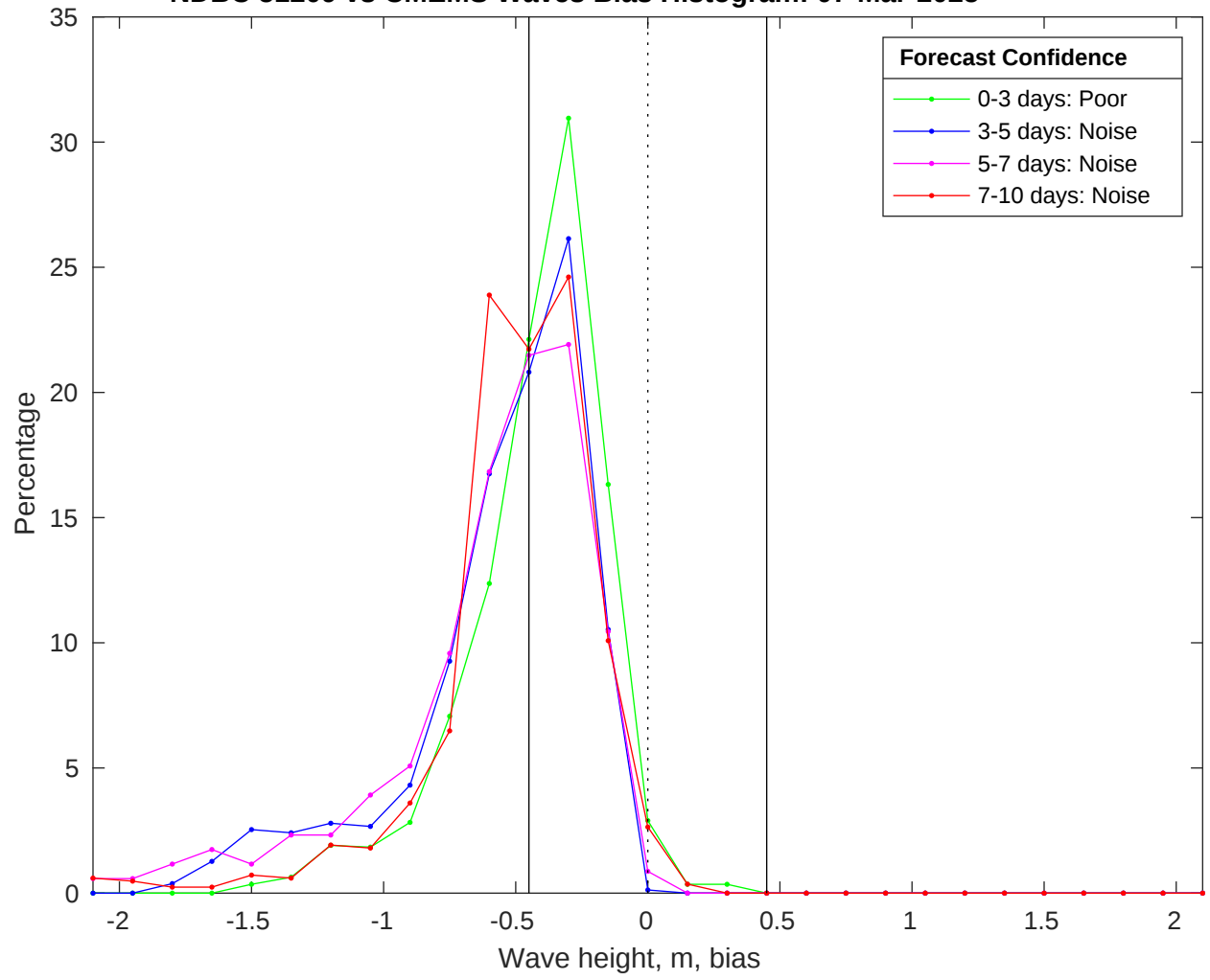
NDBC 51209 vs CMEMS Waves Bias Histogram: 07-Mar-2025
