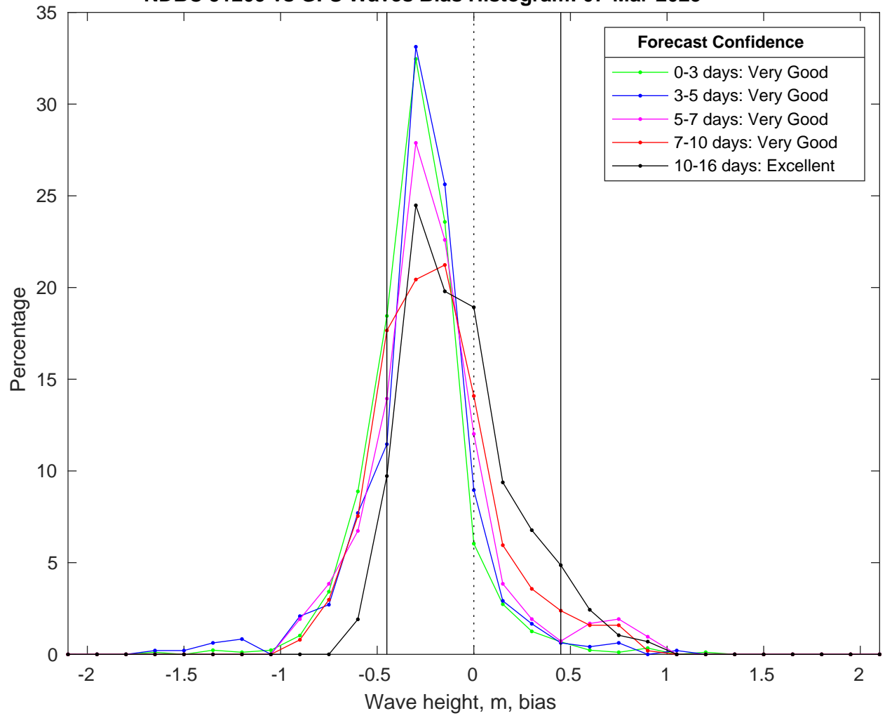
NDBC 51209 vs GFS Waves Bias Histogram: 07-Mar-2025
