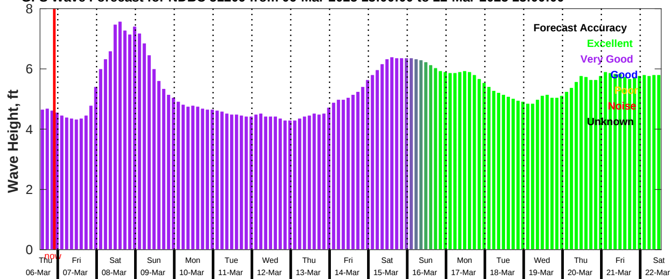
GFS Wave Forecast for NDBC 51209 from 06-Mar-2025 13:00:00 to 22-Mar-2025 13:00:00
