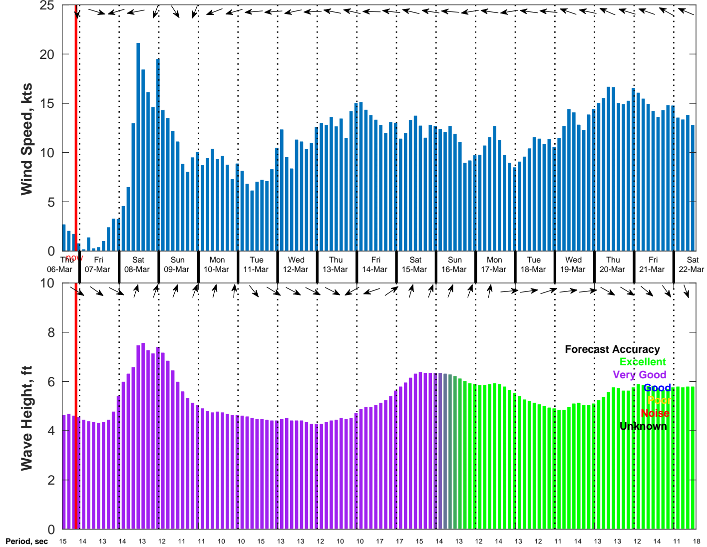
Wind & Wave Forecast for NDBC 51209 from 06-Mar-2025 13:00:00 to 22-Mar-2025 13:00:00
