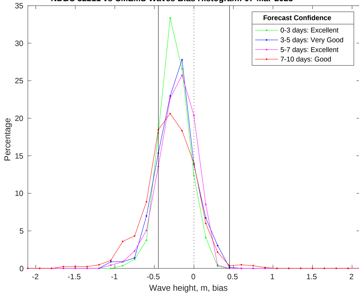
NDBC 52211 vs CMEMS Waves Bias Histogram: 07-Mar-2025
