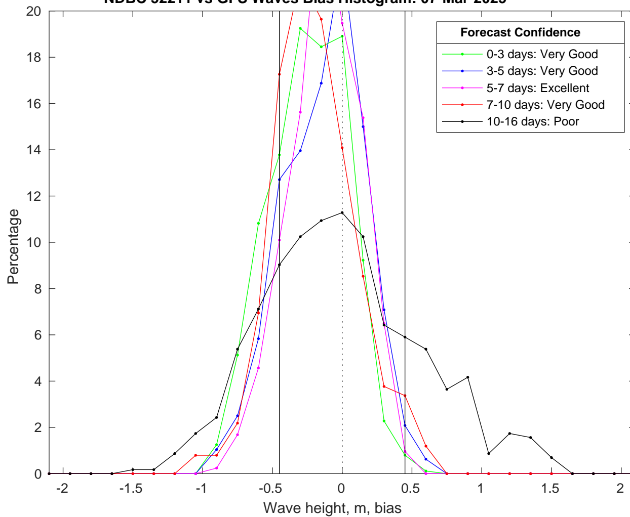
NDBC 52211 vs GFS Waves Bias Histogram: 07-Mar-2025
