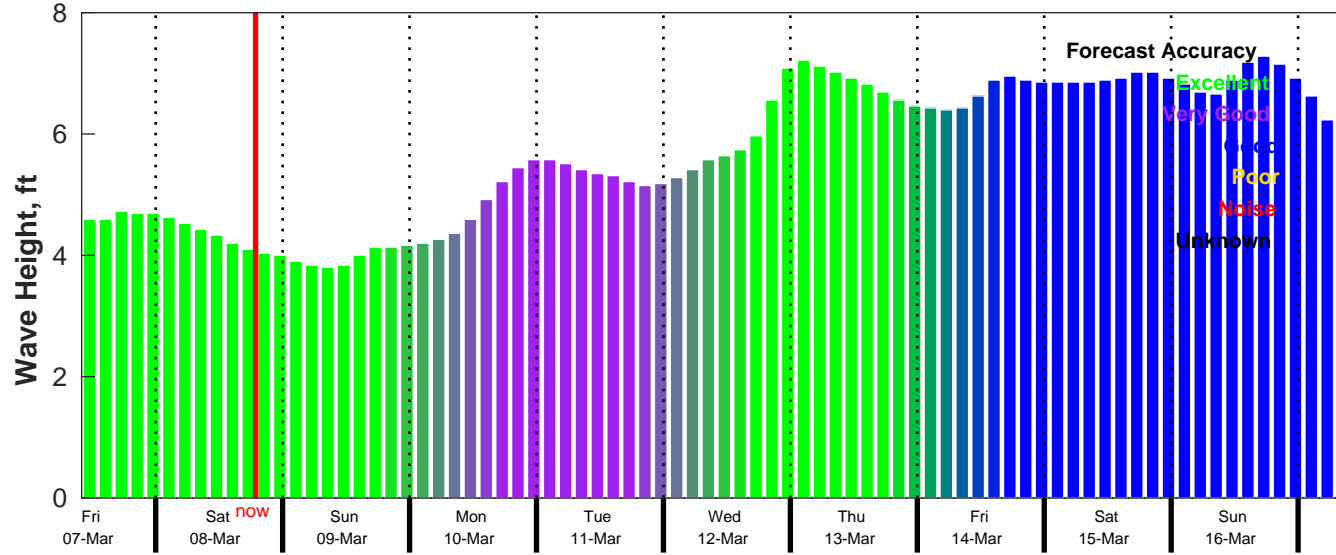
CMEMS Wave Forecast for NDBC 52211 from 06-Mar-2025 10:00:00 to 16-Mar-2025 10:00:00
