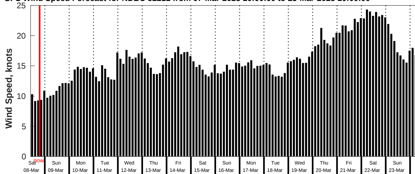
GFS Wind Speed Forecast for NDBC 52211 from 07-Mar-2025 10:00:00 to 23-Mar-2025 10:00:00
