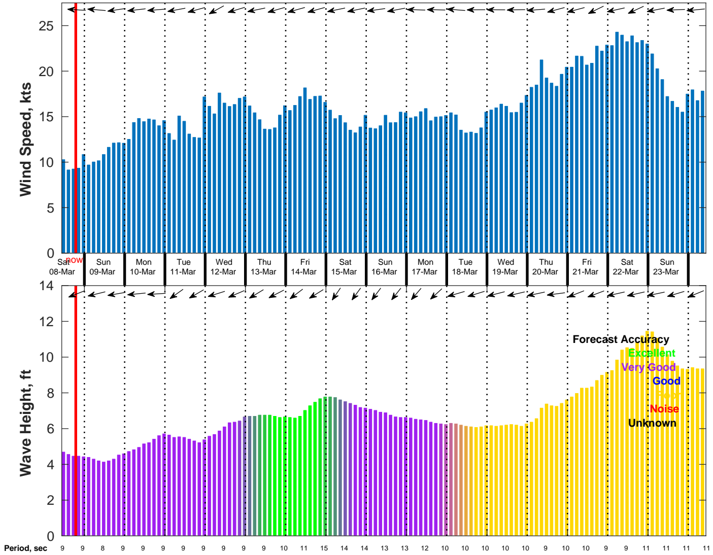
Wind & Wave Forecast for NDBC 52211 from 07-Mar-2025 10:00:00 to 23-Mar-2025 10:00:00
