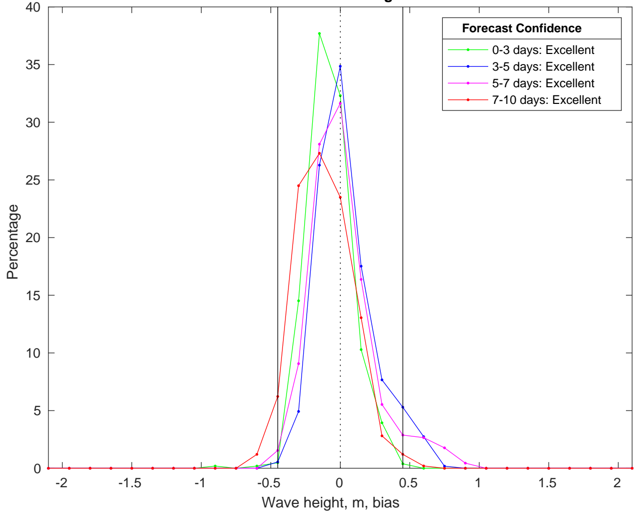
NDBC 52212 vs CMEMS Waves Bias Histogram: 07-Mar-2025
