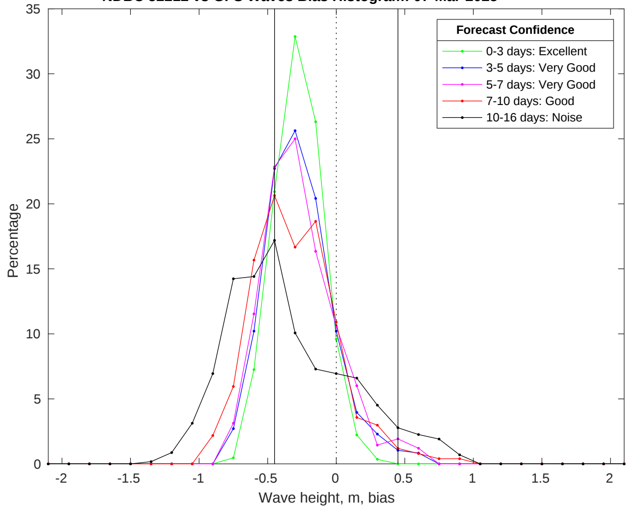
NDBC 52212 vs GFS Waves Bias Histogram: 07-Mar-2025
