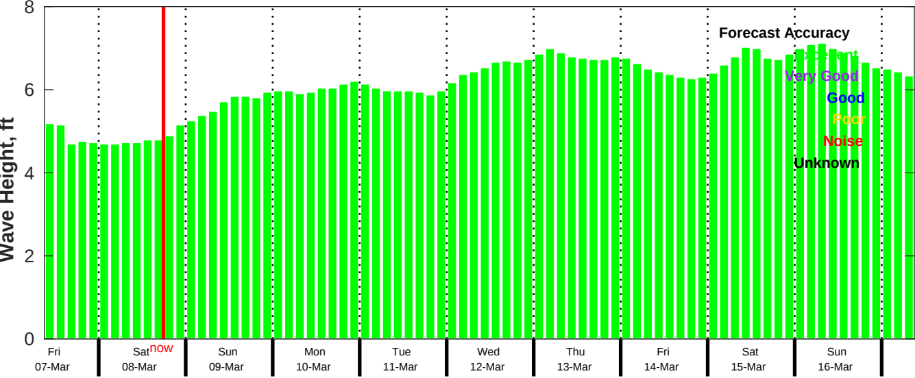
CMEMS Wave Forecast for NDBC 52212 from 06-Mar-2025 09:00:00 to 16-Mar-2025 09:00:00
