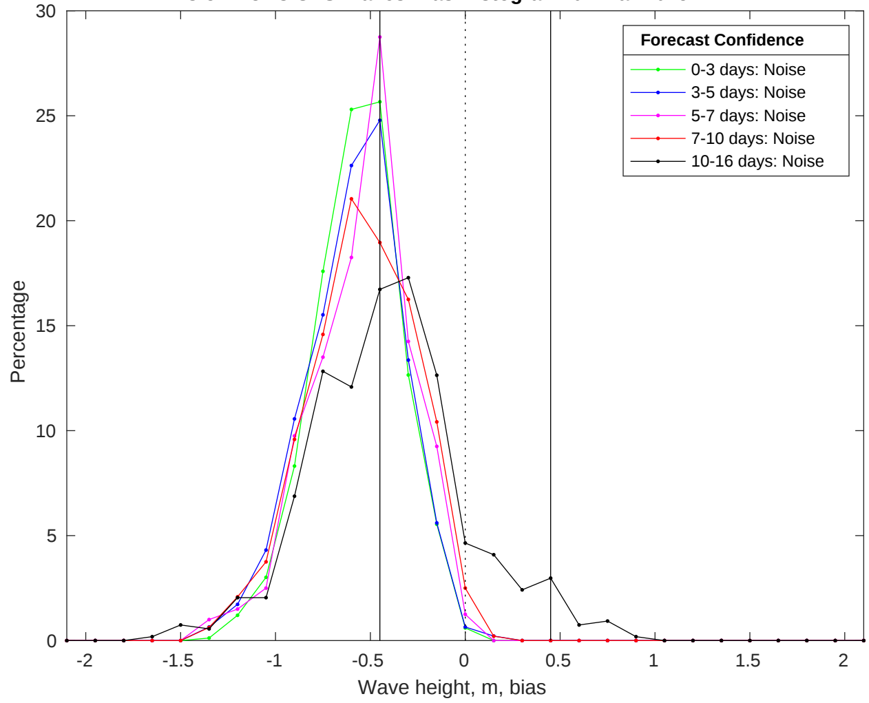
NDBC 52213 vs GFS Waves Bias Histogram: 07-Mar-2025
