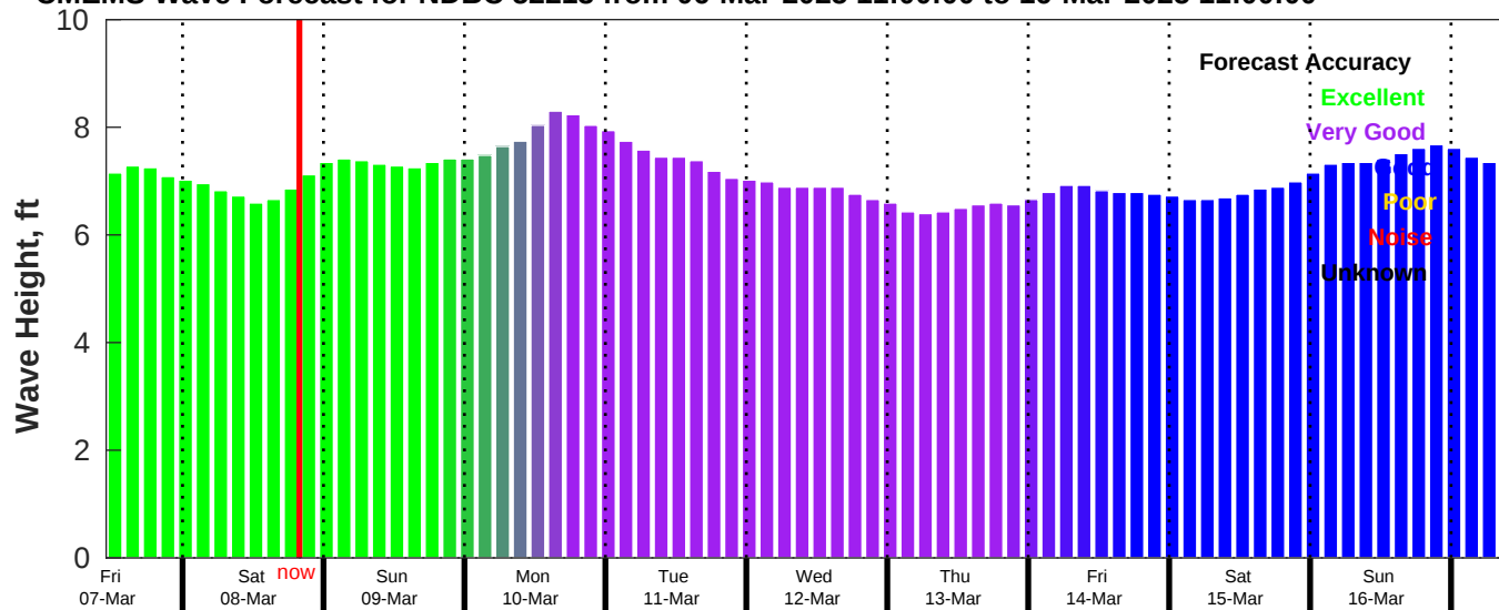
CMEMS Wave Forecast for NDBC 52213 from 06-Mar-2025 11:00:00 to 16-Mar-2025 11:00:00
