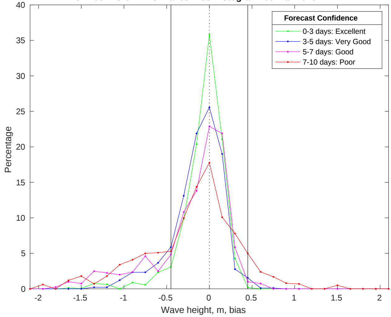
NDBC 41004 vs CMEMS Waves Bias Histogram: 08-Mar-2025
