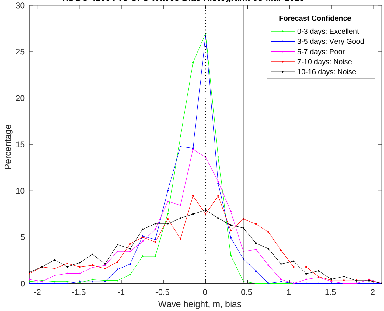
NDBC 41004 vs GFS Waves Bias Histogram: 08-Mar-2025
