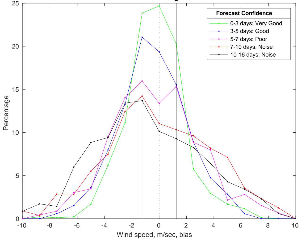
NDBC 41004 vs GFS Winds Bias Histogram: 08-Mar-2025
