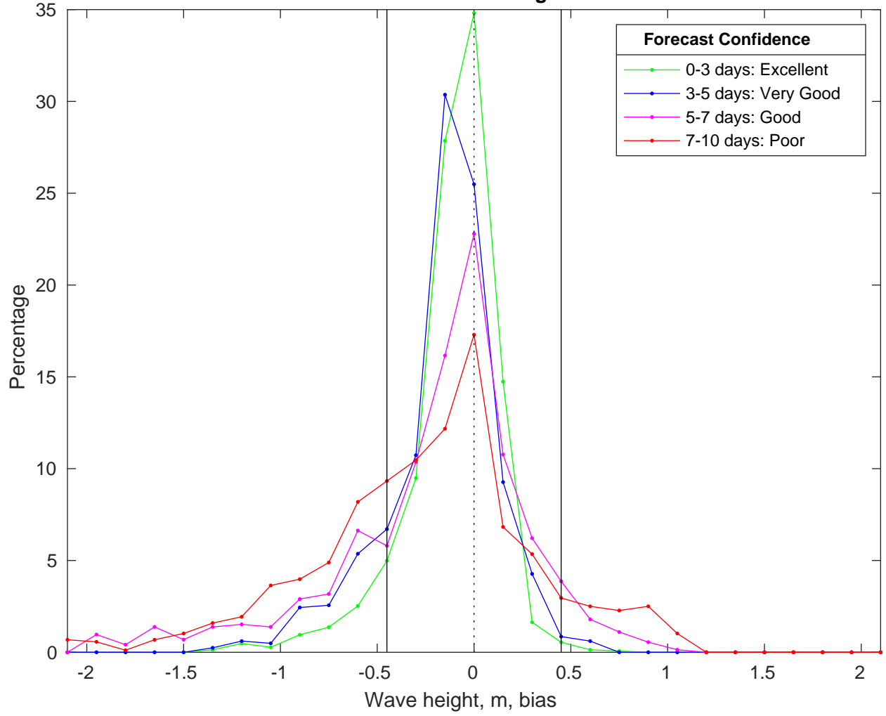
NDBC 41013 vs CMEMS Waves Bias Histogram: 08-Mar-2025
